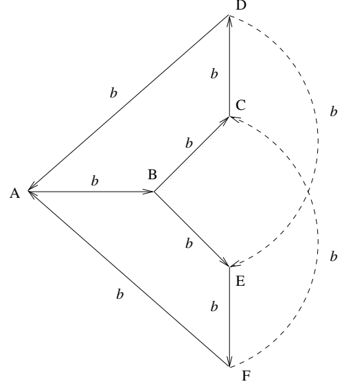
Figure 2: An order graph. Letters on edges represent order prices.
