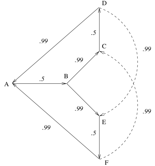
Figure 1: Every cycle has negative worst-case profit of -0.02 (for the cycles of length 4) or less (for the cycles of length 6), however accepting all edges in full gives a positive worst-case profit of 0.44.
