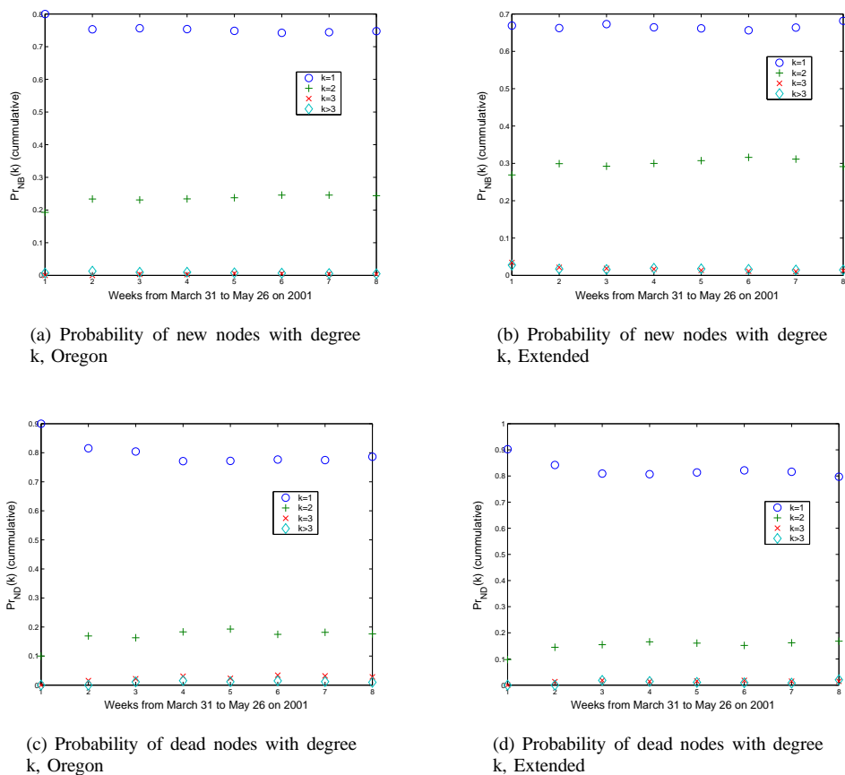
Fig. 3. Node birth vs node death : (a) and (b); About 75% of new nodes has degree one and 25% of nodes are added with degree two in the Oregon topologies. In the Extended topologies, About 70% of new nodes has degree one and 30% of nodes has degree two. In both cases, probability of new nodes with degree more than two is negligible. (c) and (d); In both cases, more than 96% of dead nodes has degree less than three. In both topologies, number of nodes with degree one is less than number of degree two nodes. All measures are consistent over time.
