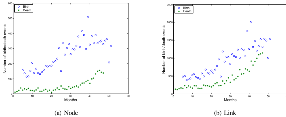
Fig. 7. Birth/death events. To avoid miscategorizing temporary node/link failures as node/link deaths, we only consider a node/link dead if it does not reappear at any time in the future in our data set. Also, we consider a node/link new only if it does not appear in any previous month. To keep the number of false dead nodes low, we do not calculate death events for the final five months. Similarly, birth events are not calculated for first five months. Our results suggest that the effect of link death cannot be ignored.
